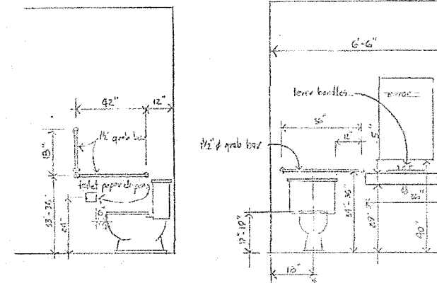
RESTROOM ELEVATIONS (1/2")
