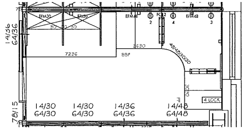
PLAN VIEW 1/4" = 1'-0"
