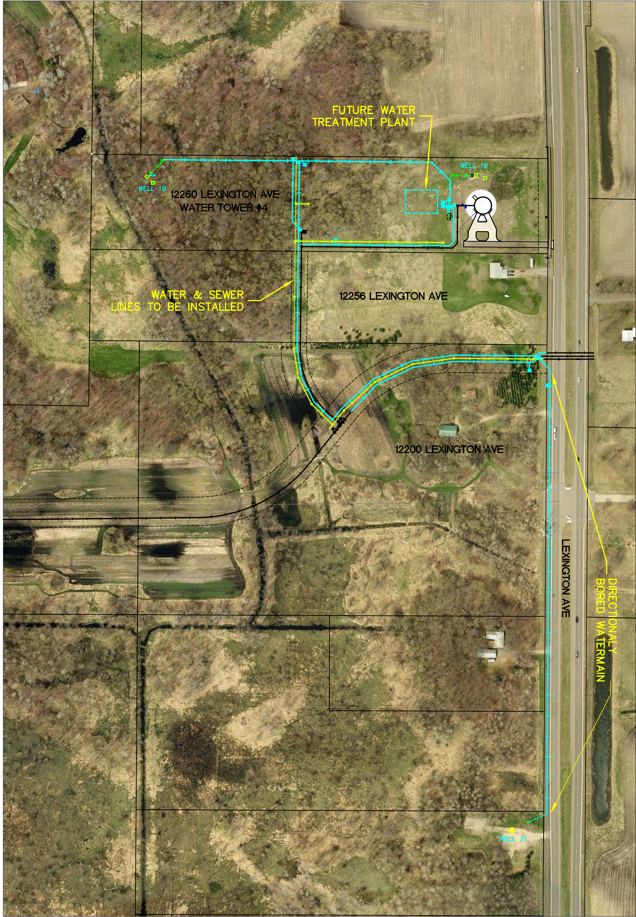
TRUNK WATERMAIN AND SANITARY SEWER FOR NE AREA WELL FIELD PROJECT LOCATION MAP
